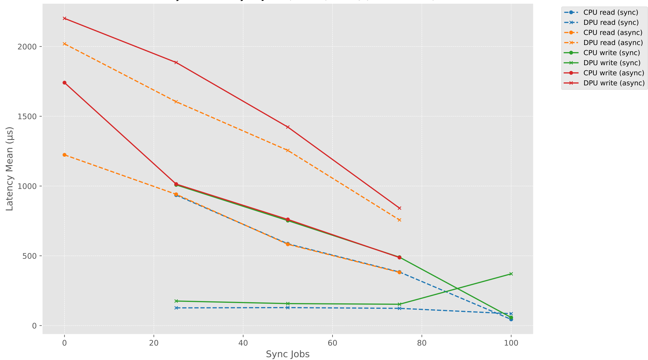
Latency Mean vs Sync Jobs (mixed) - SEQ (CPU vs DPU)
